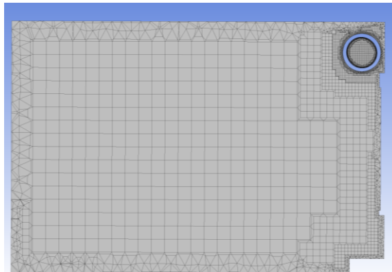
Figure 10: Tunnel cross-section at a jetfan location (with 3D CFD meshing)
