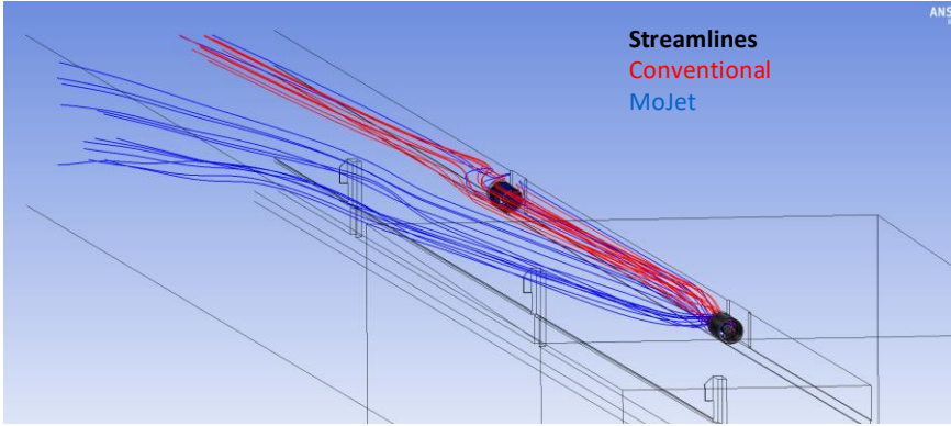
Figure 11: CFD-computed streamlines originating from conventional jetfans and MoJets
