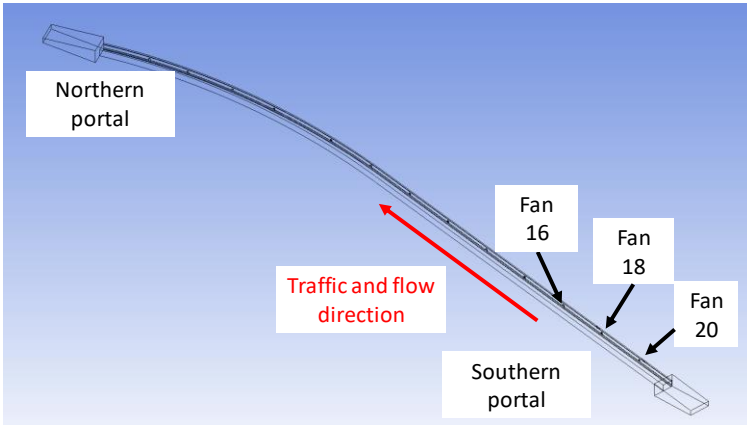
Figure 6: Location of test jettans within the Montgomery Tunnel
