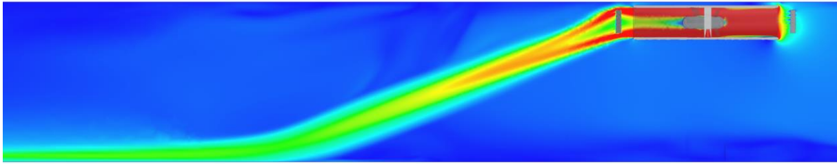
Figure 9: Velocity Contours with Deflectors (from Tarada and Else (2018))
