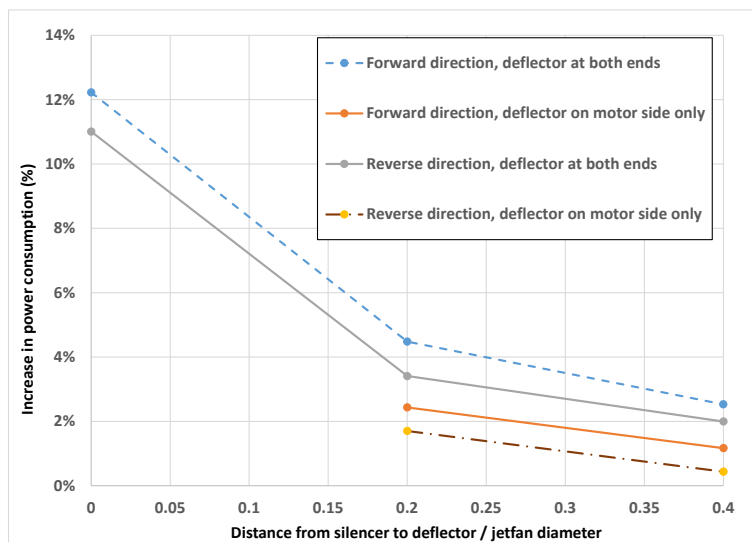
Figure 7: Increase in Motor Input Power as a Function of Deflector Location
